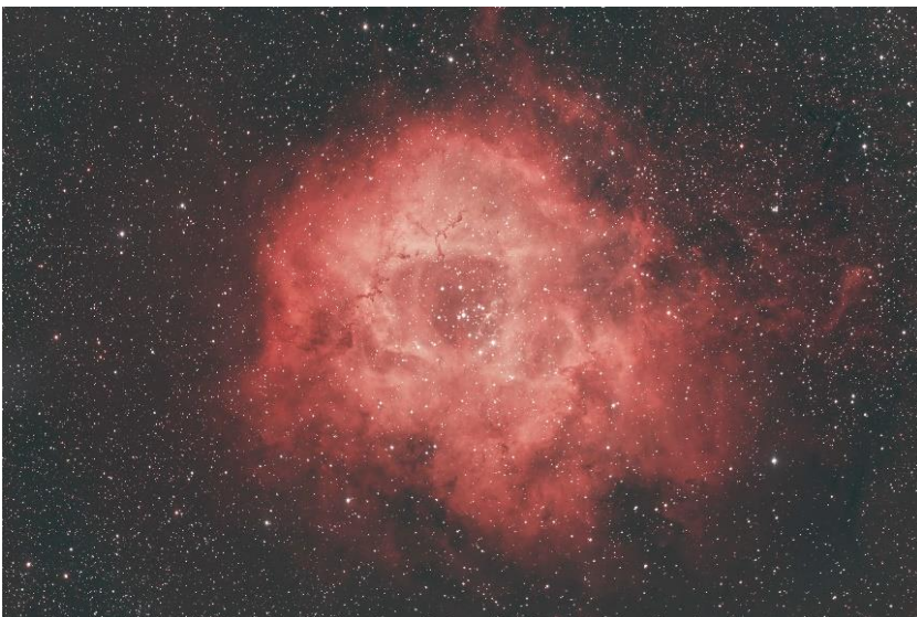
NGC 2237 (Rosette Nebula) – 20 300sec. exp. – OSC CMOS camera
