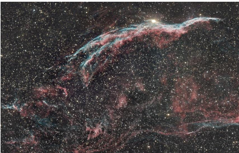
NGC 6960 (Witch's Broom) – 37 300sec.exp. – OSC CMOS camera
