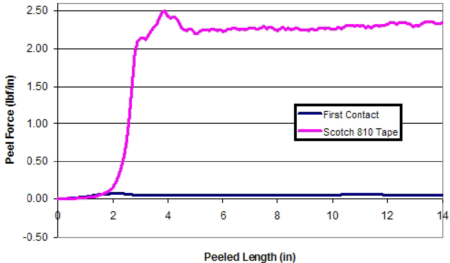
First Contact vs Scotch Tape (810) Peel from Borofloat Glass First Surface Aluminum Mirror
